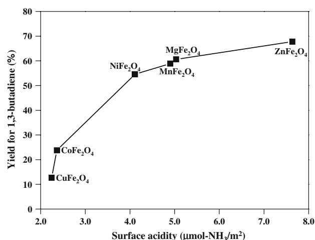
Fig. 5 A correlation between yield for 1,3-butadiene and surface acidity of metal ferrite catalysts
